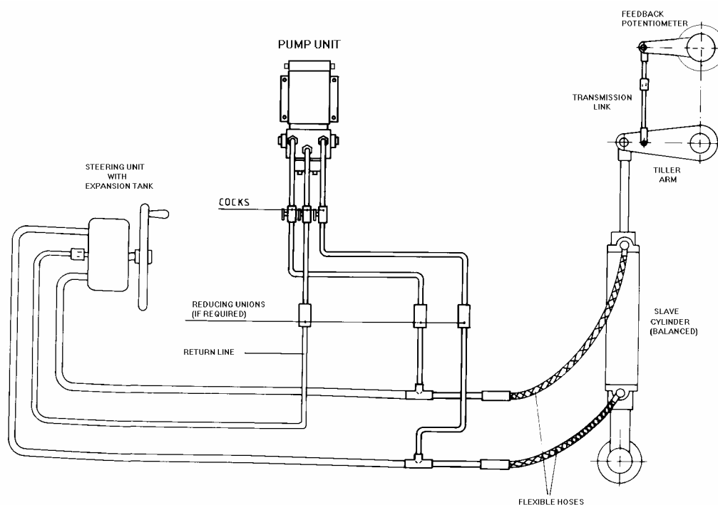
Figure 4-5 Connection to hand hydraulic steering gear Drw.no. 3-110101
